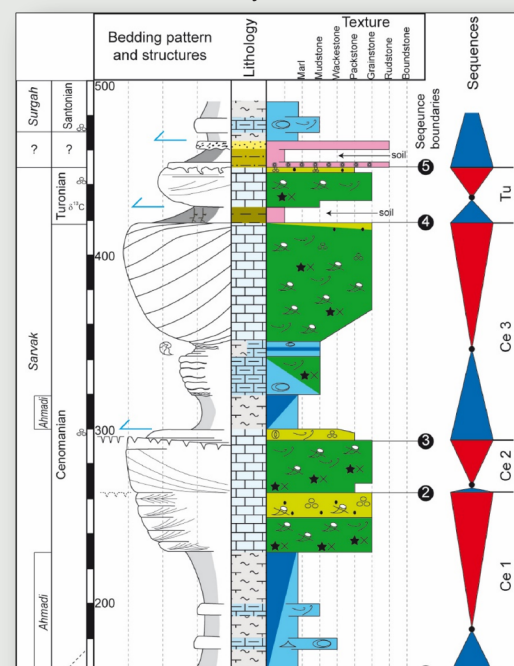
Cenomanian Sarvak cycles
